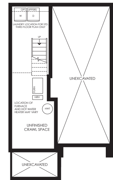
CRAWL SPACE PLAN ELEV. 'A', 'B'
