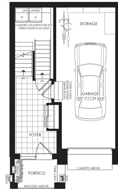
GROUND FLOOR PLAN ELEV. 'A', 'B'
