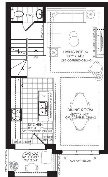
SECOND FLOOR PLAN ELEV. 'A', 'B'
