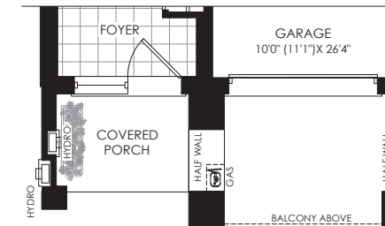
PARTIAL GROUND FLOOR PLAN ELEV. 'F'
