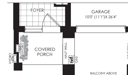
PARTIAL GROUND FLOOR PLAN ELEV. 'G'
