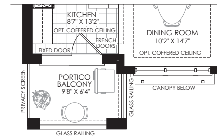
PARTIAL SECOND FLOOR PLAN ELEV. 'C'
