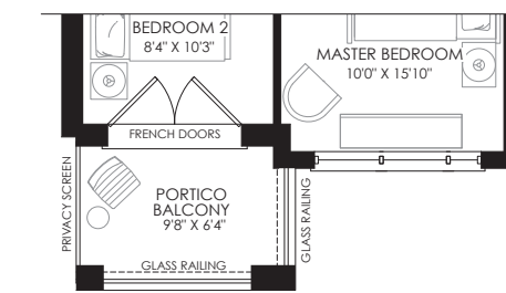
PARTIAL THIRD FLOOR PLAN & THIRD FLOOR FLEX PLAN ELEV. 'C' WITH ROOF TOP TERRACE
